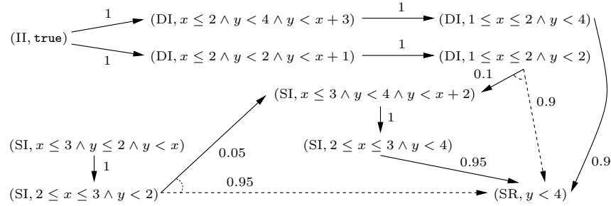
Fig. 3. The probabilistic system generated by ProbReach for the PTA in Figure 1.
